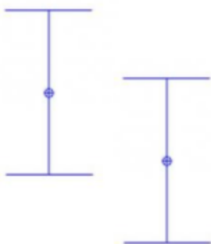
Overlapping Confidence Intervals, Subgroup Not Identified
