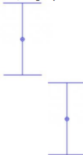
Non-overlapping Confidence Intervals, Subgroup Identified
